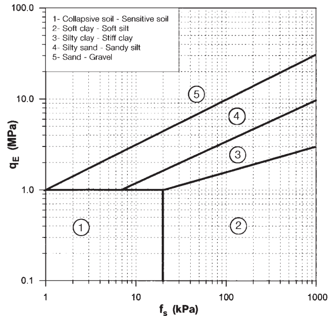
Fig. 2. New soil profiling chart.
